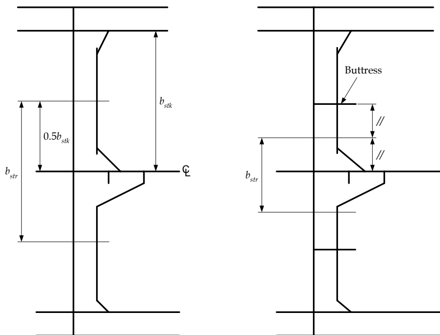
Figure 8.1.7 Load Breadth of Stringers for Ships with a Centreline Bulkhead
