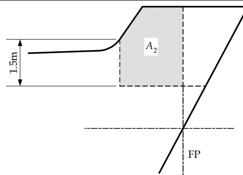
Figure 11.4.2 Profile Areas of Screens and Bulwarks
