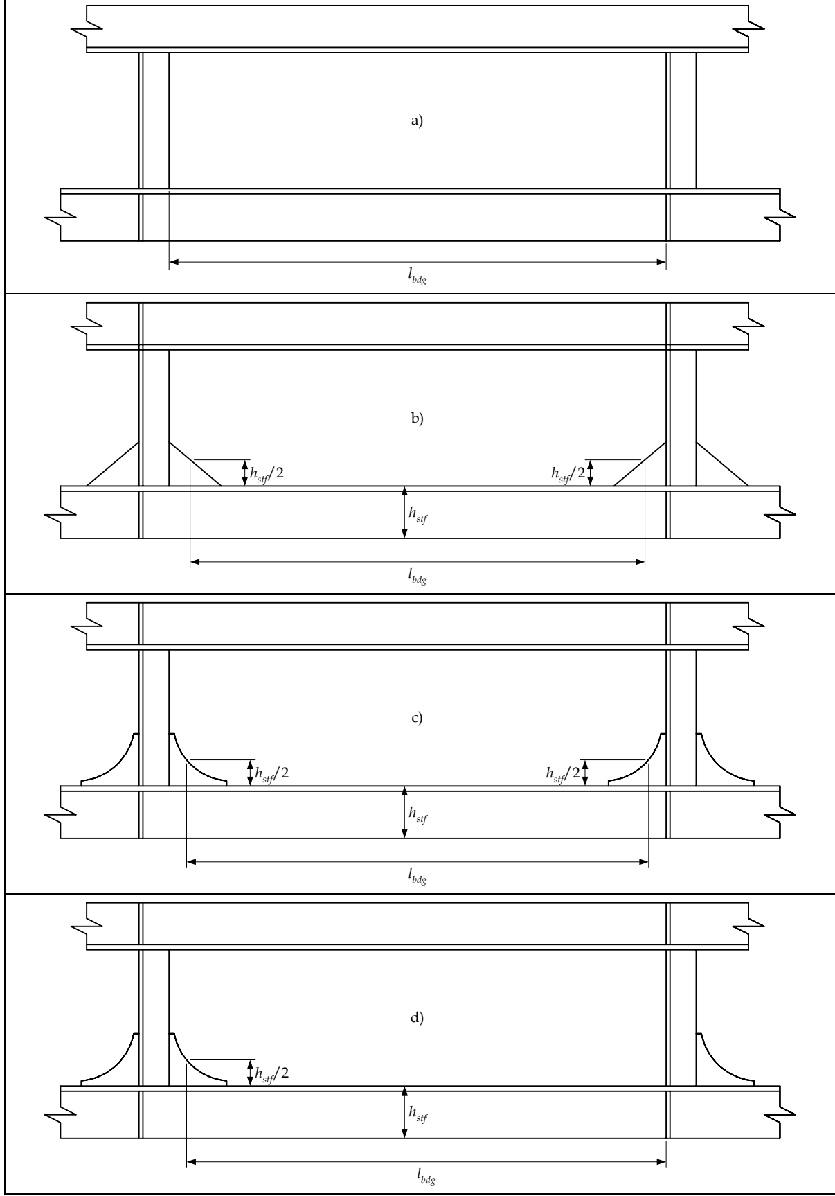
Figure 4.2.1 Effective Bending Span of Stiffeners Supported by Web Stiffeners (Double Skin Construction)
