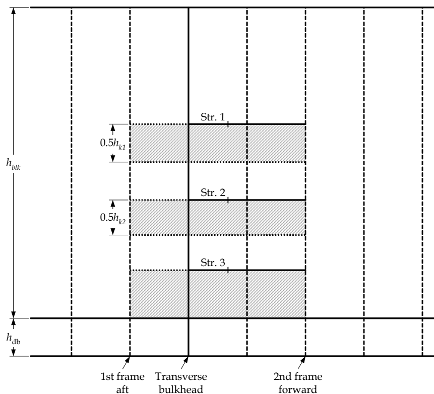
Figure 8.1.6 Region for Stringer Correction, t_{ij} , for a Tanker with Three Stringers
