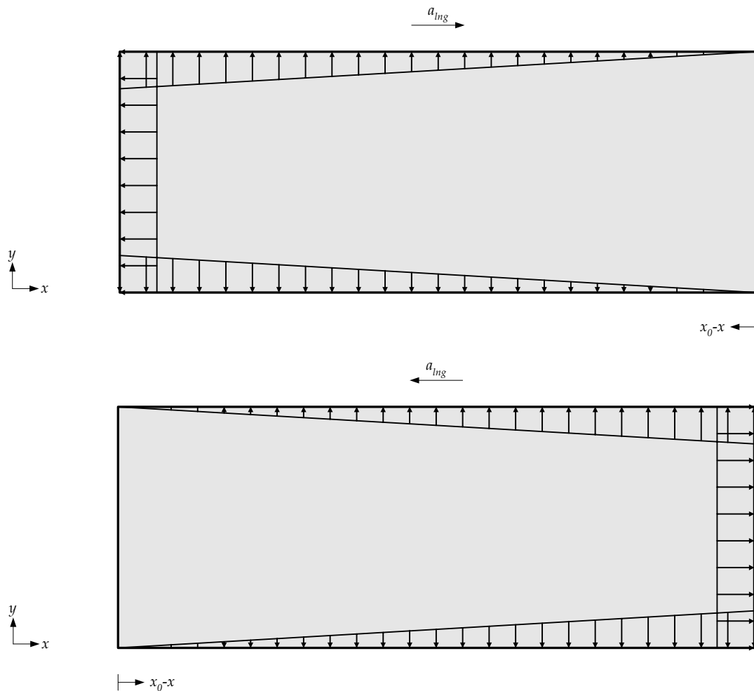
Figure 7.6.6 Dynamic Tank Pressure in Tanks due to Positive and Negative Longitudinal Acceleration
